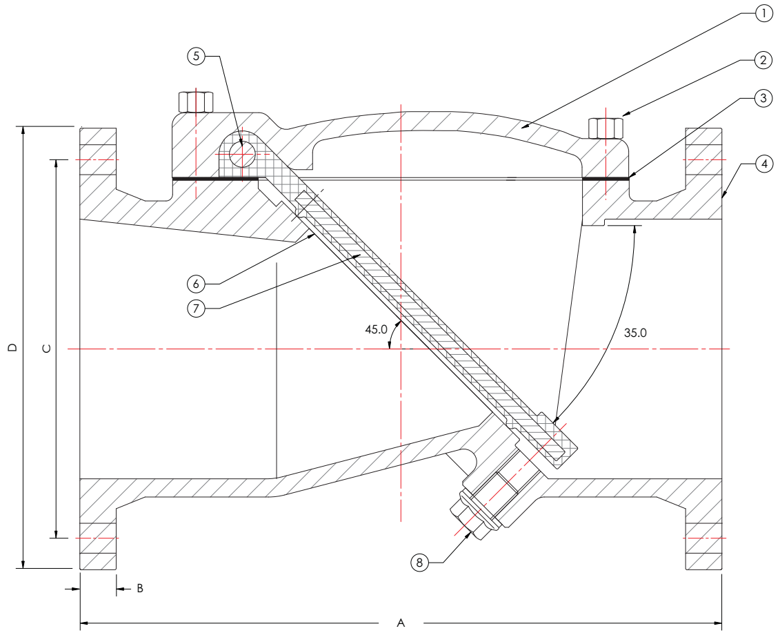
4" - 24" C508 Rubber Flapper Check Valve (FLxFL)
